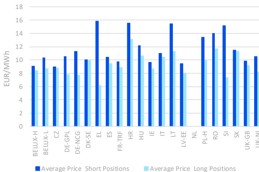
Figure 9: Average buy-sell spread on imbalance cash out prices
