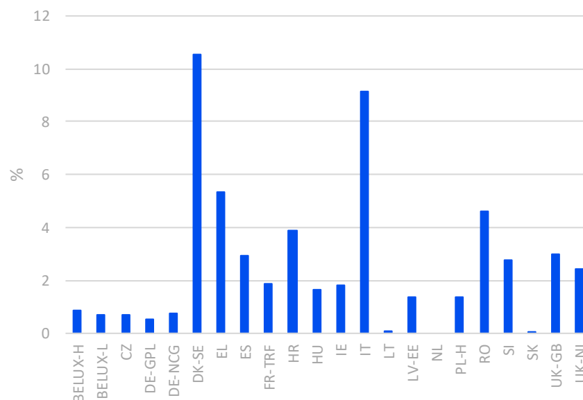
Figure 7: Total imbalance quantities as a share of market volume
